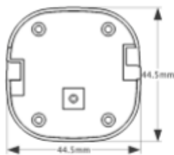
BOX120W(No bracket)
